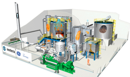
Figure 4: Configuration of 2 MWe IC Engine Based CHP System
